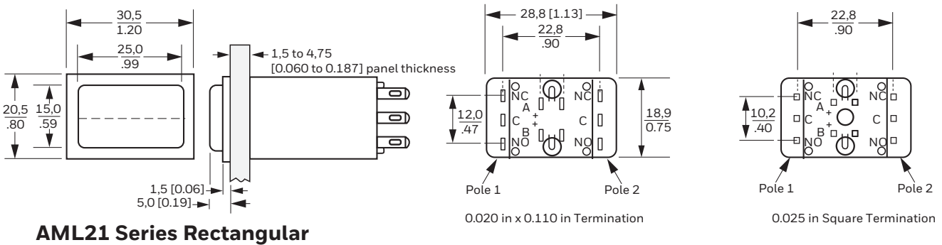
AML21 Series Square
