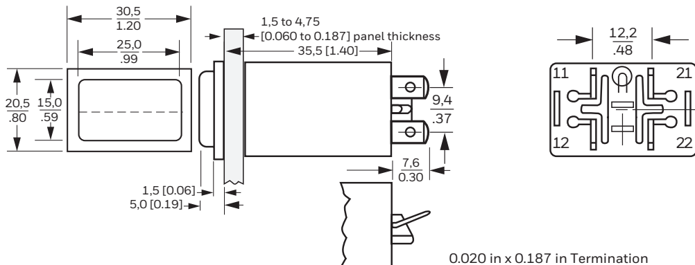
AML31 Series Rectangular
