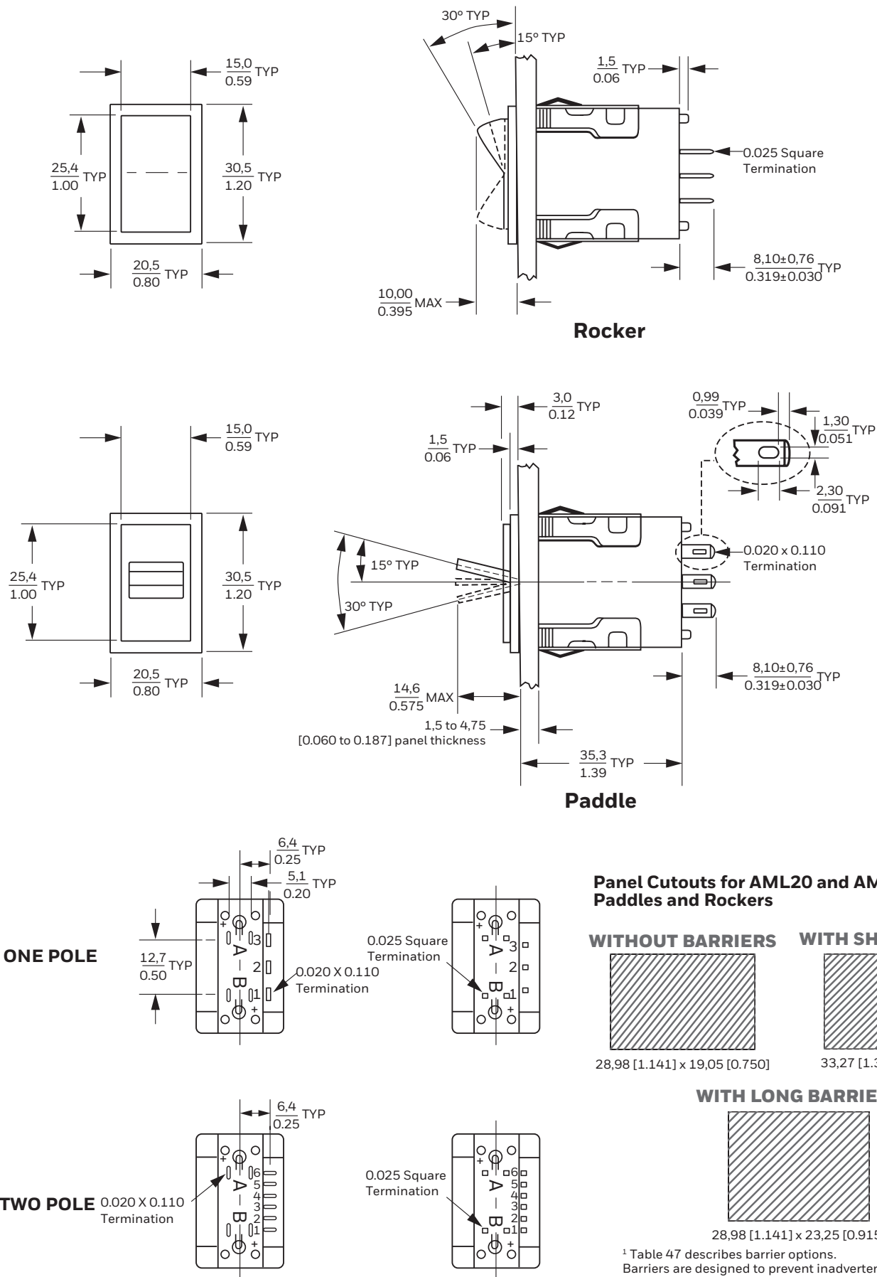
Figure 23. AML23 and AML24 Series Dimensions mm [in] or mm\in
