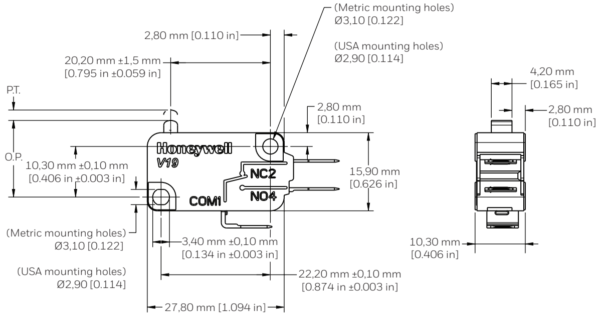
FIGURE 4. V19 SERIES HOUSING DIMENSIONS
